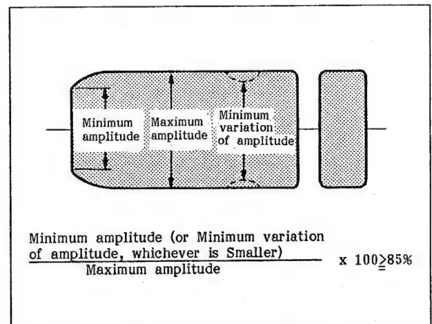
Fig. 5-17 Tracking Check
